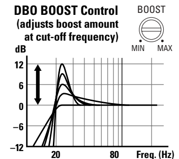
Figure 13. Frequency response curves show typical DBO control ranges for the JBL A6000GTi or A3000GTi amplifier.
